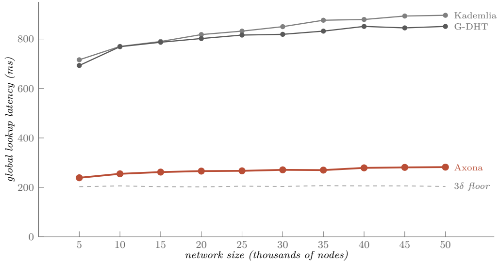
Figure 4: Global lookup latency versus network size at every 5,000 from 5,000 to 50,000 nodes ( 10\times scaling), plotted against the Dabek 3\delta analytical floor (gray dashed). Kademia climbs from 716 to 896 ms as the log- N hop tax compounds; G-DHT tracks Kademia almost identically on global lookups (the geographic prefix only helps regional cells). Axona hugs the floor in a tight 239–282 ms band across the whole range ( 1.17\text{--}1.38\times the 3\delta floor) and is essentially flat from 15,000 nodes onward — adding 35,000 more nodes raises latency by 20 ms total. All success rates 100%. Data: sim v0.93.0 / @axona/protocol v1.1.3, May 2026.
